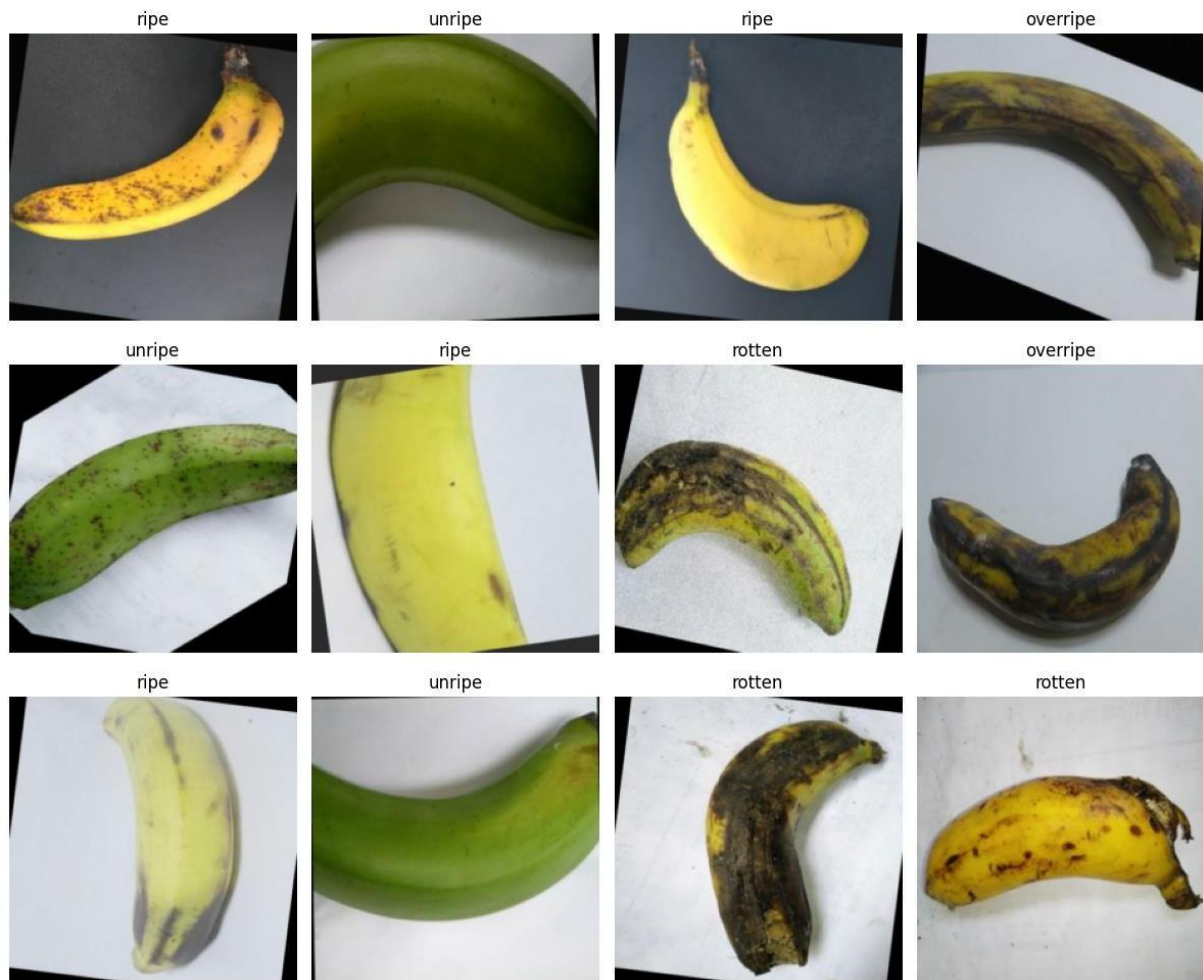
Figure 1. Dataset Banana
