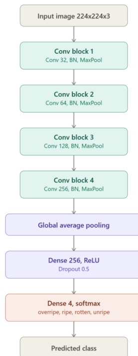
Figure 2. CNN-from-scratch architecture
